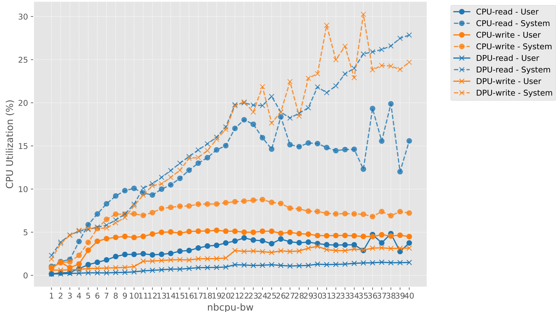
CPU Utilization vs nbcpu-bw (CPU vs DPU)
